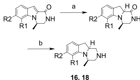
Scheme 3. Reagents and conditions: (a) Mg, MeOH; (b) LiAlH 4 , THF, reflux.
