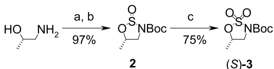
Scheme 1. Reagents and conditions: (a) (Boc) 2 O, CH 2 Cl 2 ; (b) SOCl 2 , imidazole, CH 2 Cl 2 , –50 °C; (c) NaIO 4 , RuO 2 , EtOAc.
