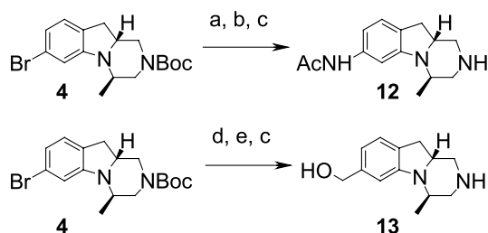
Scheme 4. Reagents and conditions: (a) \text{Pd}_2(\text{dba})_3 , ( \pm )-BINAP, NaOt-Bu, toluene, benzophenone imine; Pd/C, \text{NH}_4 -formate, MeOH; (b) AcCl, \text{NEt}_3 , \text{CH}_2\text{Cl}_2 ; (c) TFA, \text{CH}_2\text{Cl}_2 ; (d) n -BuLi, THF, \text{CO}_2 , -78^\circ\text{C} ; (e) \text{LiAlH}_4 , THF.
